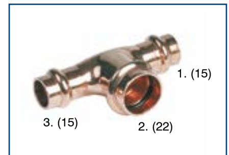
Pressfitting, T-Stück P5130 15 x 22 x 15 mm
